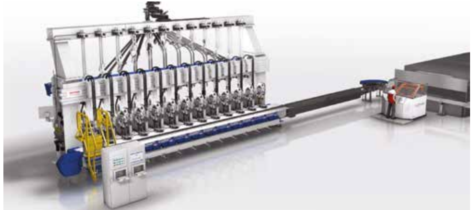
Servo ware handling with FlexPusher, FlexConveyor, servo take out and FlexIS controls.
